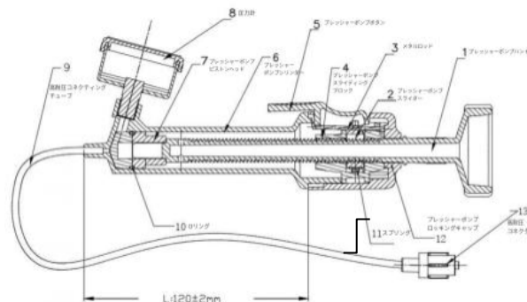
Figure 1: AGI Disposable Inflation Device II
